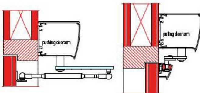
▲ cross-section KONE automatic swing doors. ▲
